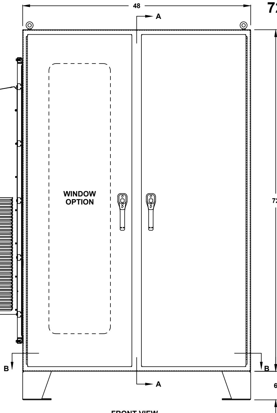
FRONT VIEW
