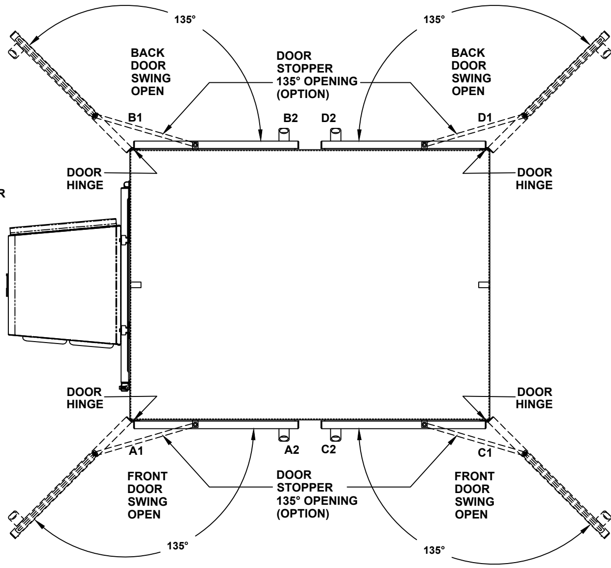
TOP VIEW
