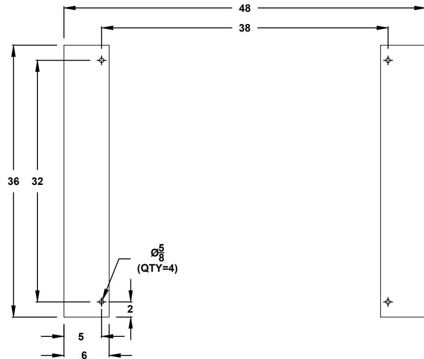
CROSS SECTION VIEW C-C MOUNTING HOLES
