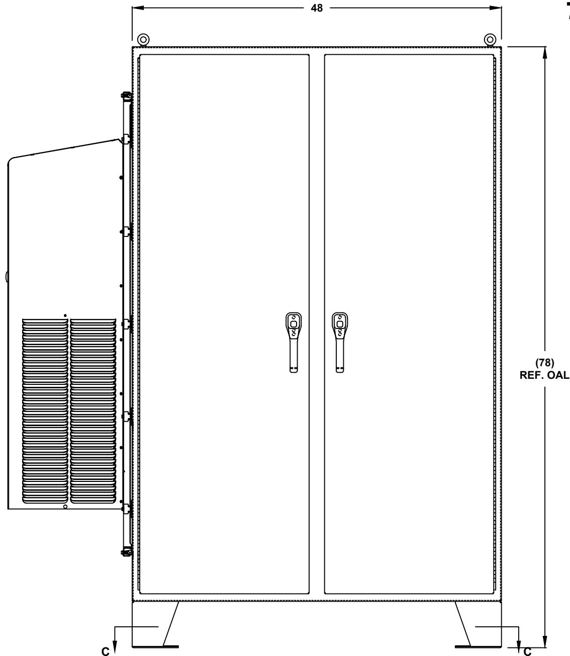
FRONT VIEW
